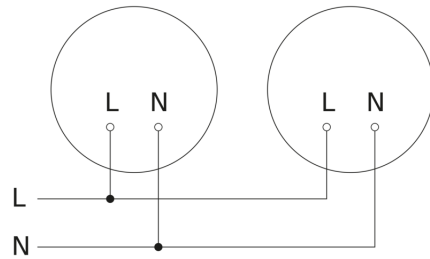
Master/master bluetooth interconnection circuit diagram
